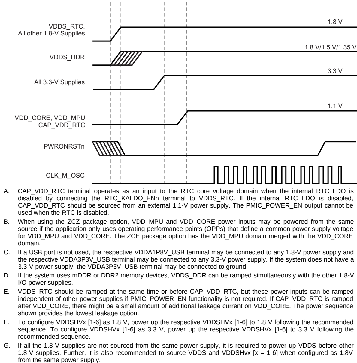
图 6-6. Power-Supply Sequencing With RTC Feature Disabled
