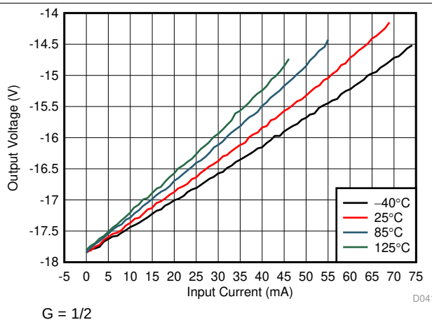
图 41. Negative Output Voltage vs Output Current (Sinking)
