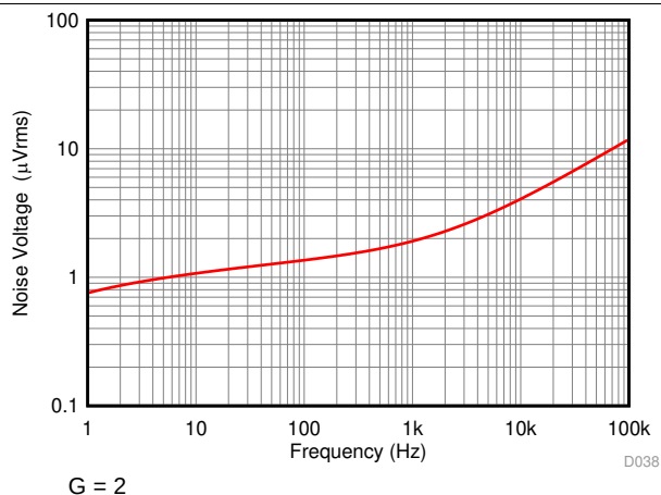
图 38. Integrated Output Voltage Noise vs Noise Bandwidth
