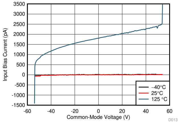
图 13. Input Bias Current vs Common-Mode Voltage
