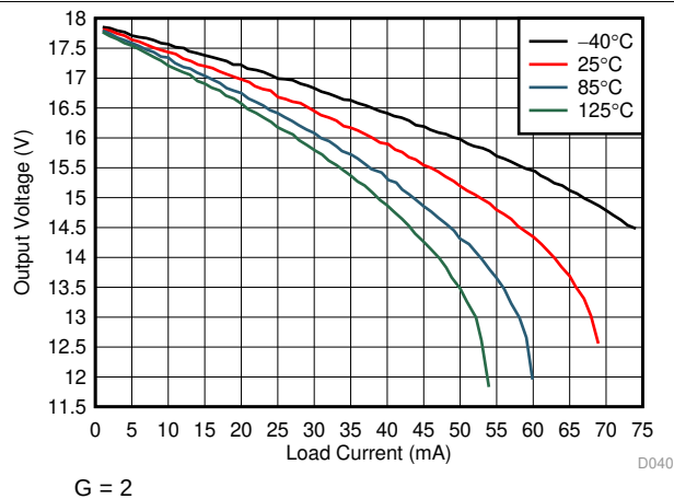
图 40. Positive Output Voltage vs Output Current (Sourcing)
