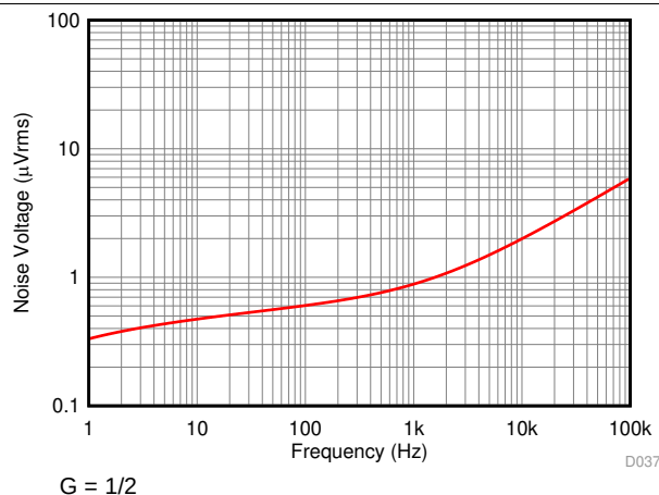
图 37. Integrated Output Voltage Noise vs Noise Bandwidth
