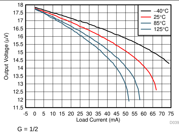
图 39. Positive Output Voltage vs Output Current (Sourcing)
