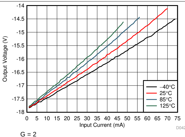
图 42. Negative Output Voltage vs Output Current (Sinking)
