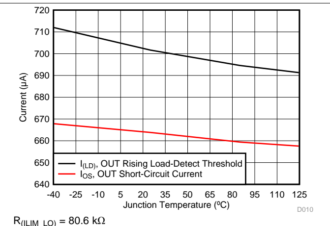
Figure 10. I_{OUT} Rising Load-Detect Threshold and I_{OUT} Short-Circuit Current Limit vs Temperature
