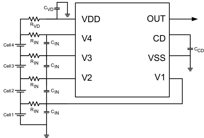
Figure 9-1. Application Configuration
