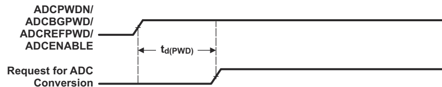
图 8-19. ADC Conversion Timing
