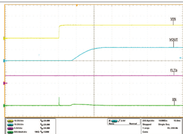
图 39. Hot Plug Response
