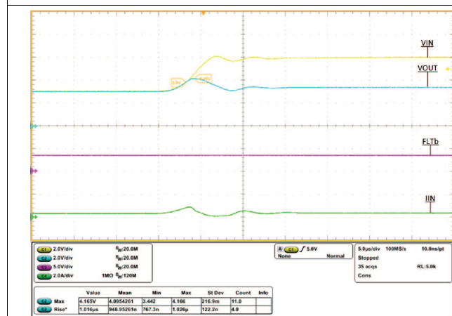
图 40. TPS259573 Overvoltage Lockout Response
