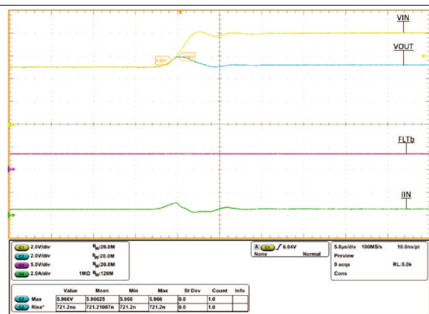
图 41. TPS259573 Overvoltage Lockout FLT Response
