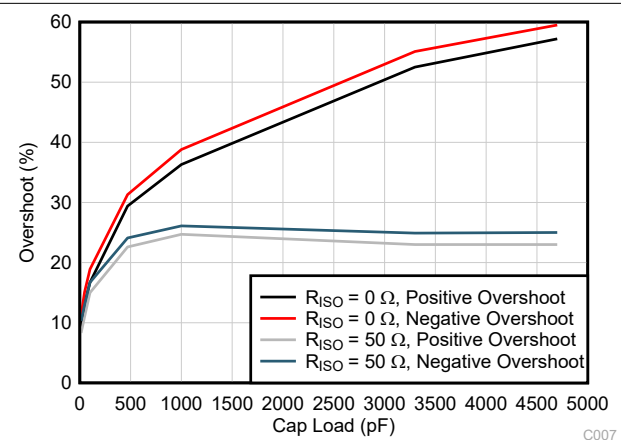
图 7-6. Small-Signal Overshoot vs Capacitive Load (100-mV Output Step, G = -1 )
