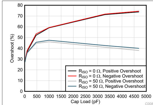
图 7-5. Small-Signal Overshoot vs Capacitive Load (100-mV Output Step, G = 1 )
