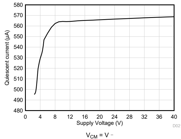
图 6-23. Quiescent Current vs Supply Voltage
