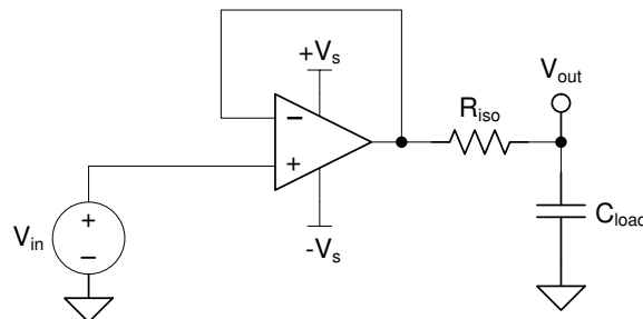
图 7-7. Extending Capacitive Load Drive With the TLV9351-Q1
