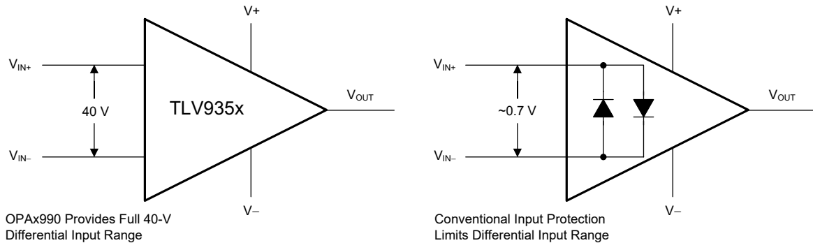
图 7-1. TLV935x-Q1 Input Protection Does Not Limit Differential Input Capability
