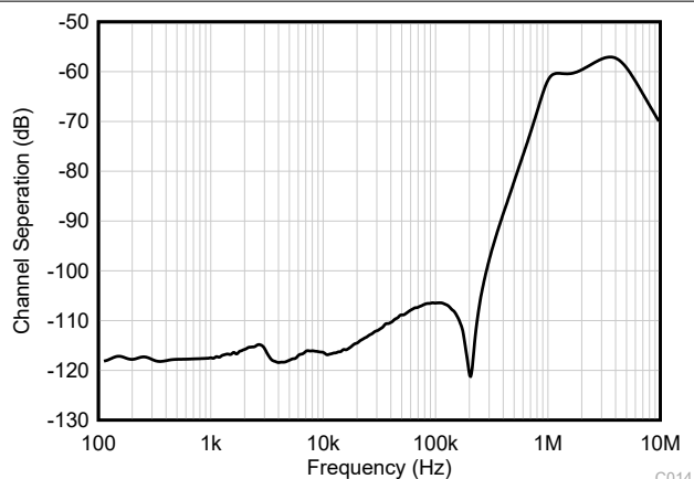
图 6-40. Channel Separation vs Frequency
