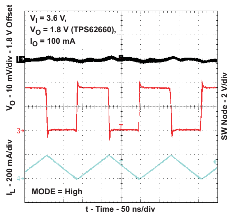
Figure 34. PWM Operation
