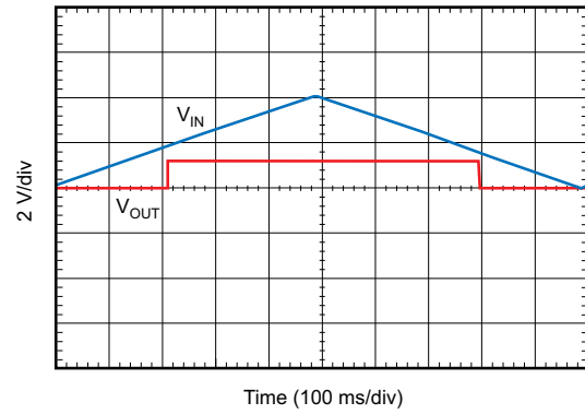
Figure 67. V_{IN} Ramp Up, Ramp Down Response
