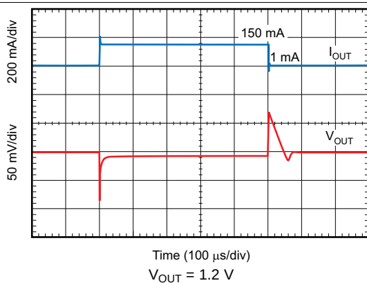
Figure 41. Load Transient Response
