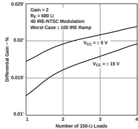
图 40. Differential Gain vs Number of 150-Ω Loads
