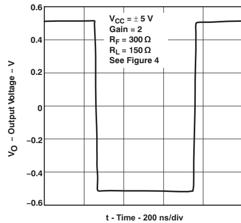
图 42. 1-V Step Response
