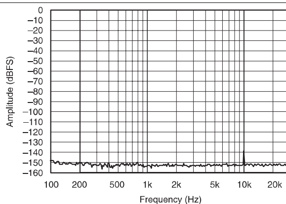
Figure 10. Crosstalk With F_{IN} = 10\text{ kHz}
