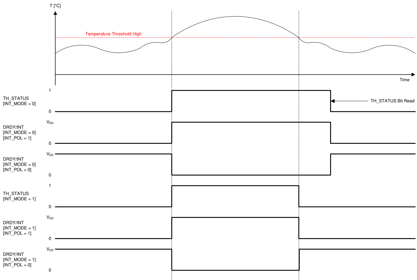
图 8-3. INTERRUPT on Threshold - Temperature High
