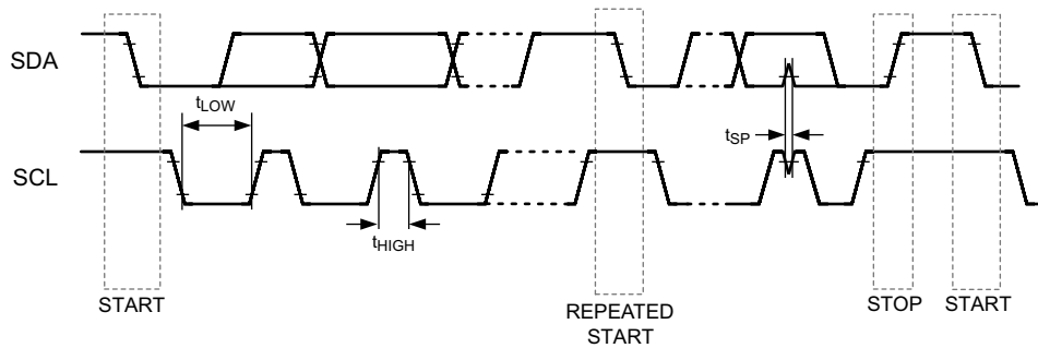
图 7-1. I2C Timing
