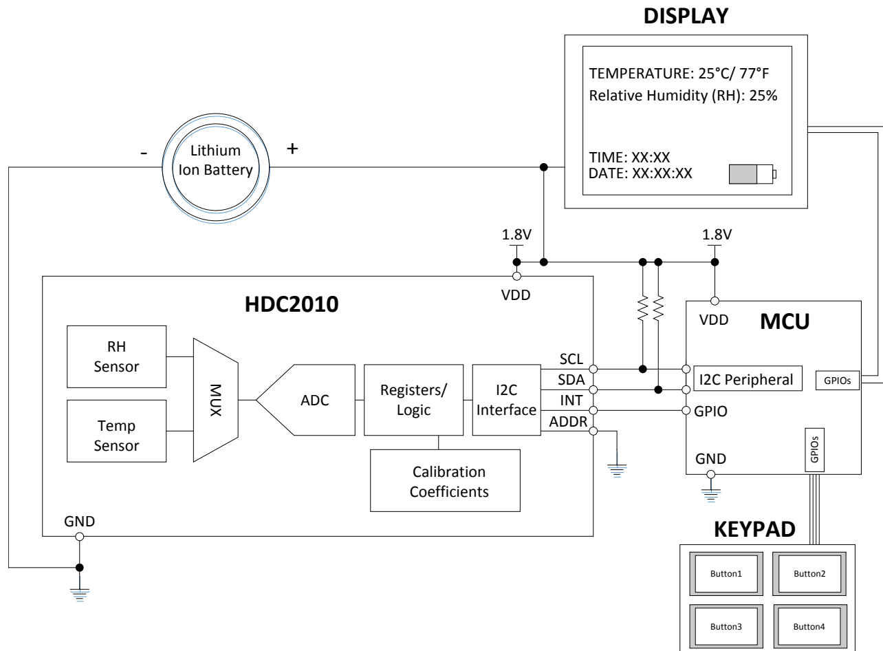
图 9-1. Typical Application Schematic HVAC
