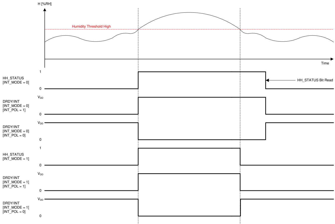
图 8-5. INTERRUPT on Threshold - Humidity High
