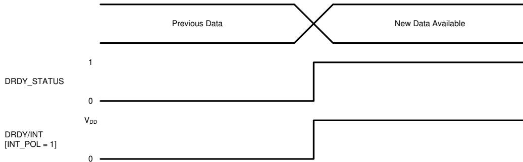
图 8-1. Data Ready Interrupt - Active High (INT_POL = 1)
