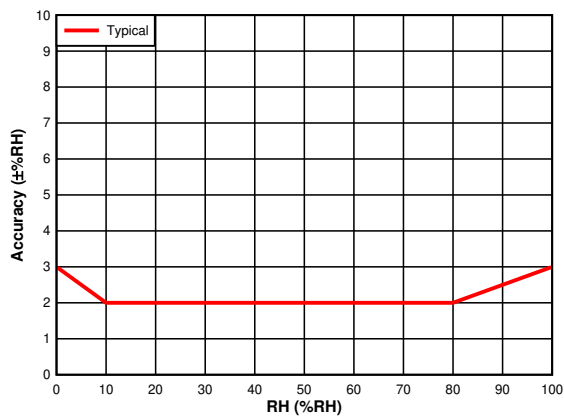
图 7-2. RH Accuracy vs. RH Set Point
