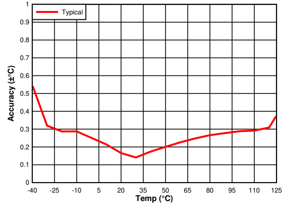
图 7-3. Temperature Accuracy vs. Temperature Set Point
