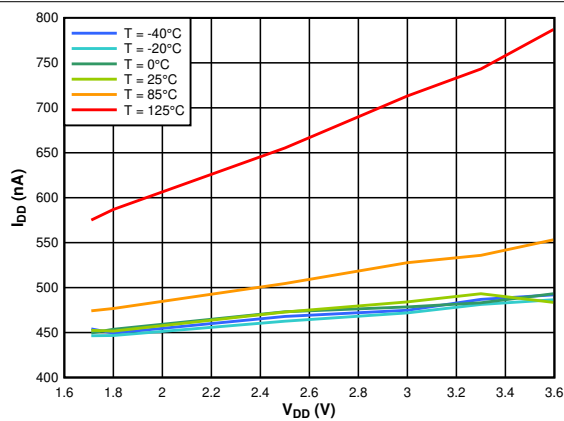
图 7-4. Supply Current vs. Supply Voltage, Average at 1 Measurement/Second, RH (11 Bit) and Temperature (11 Bit)
