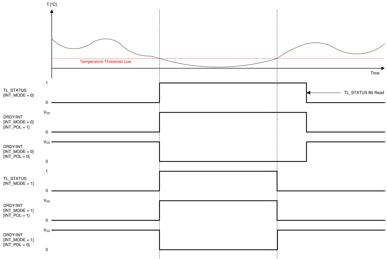
图 8-4. INTERRUPT on Threshold - Temperature Low
