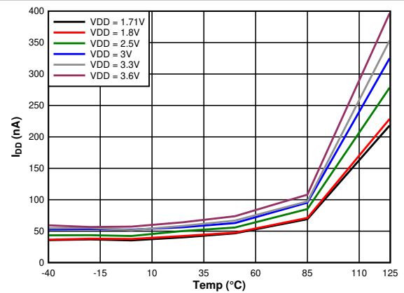
图 7-7. Supply Current vs. Temperature, Sleep Mode
