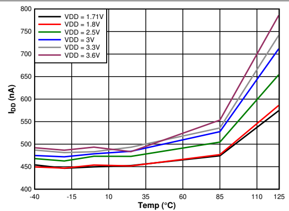
图 7-5. Supply Current vs. Temperature, Average at 1 Measurement/Second, RH (11 Bit) and Temperature (11 Bit)
