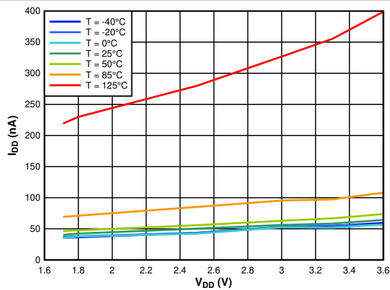
图 7-6. Supply Current vs. Supply Voltage, Sleep Mode
