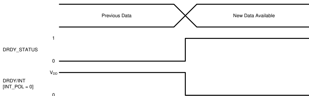
图 8-2. Data Ready Interrupt - Active Low (INT_POL = 0)
