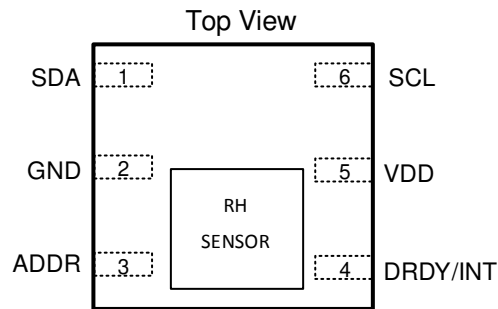
图 6-1. DMB Package 6-Pin PWSON Top View
