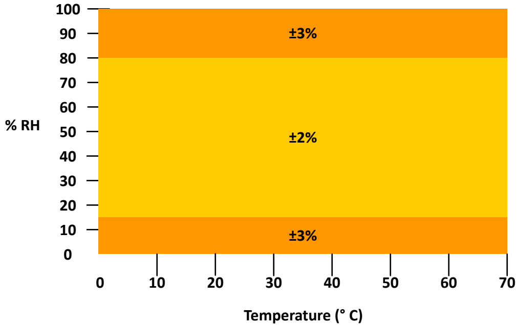
图 11-1. Typical Relative Humidity Accuracy Range Limits
