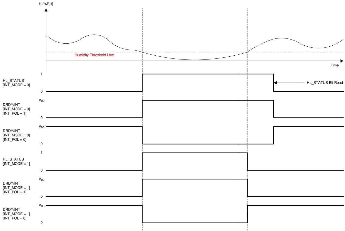
图 8-6. INTERRUPT on Threshold - Humidity Low
