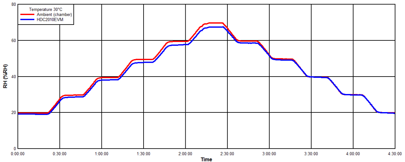
图 9-2. RH% Readings of Chamber and HDC2080 vs. Time
