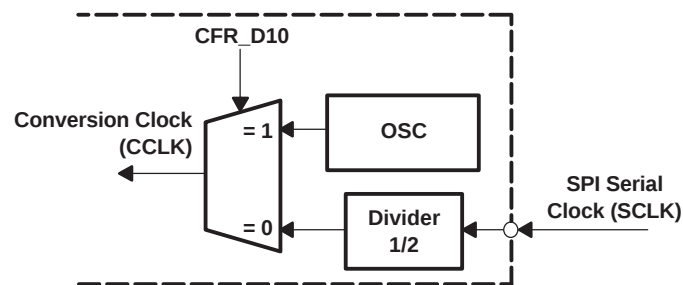
Figure 56. Converter Clock
