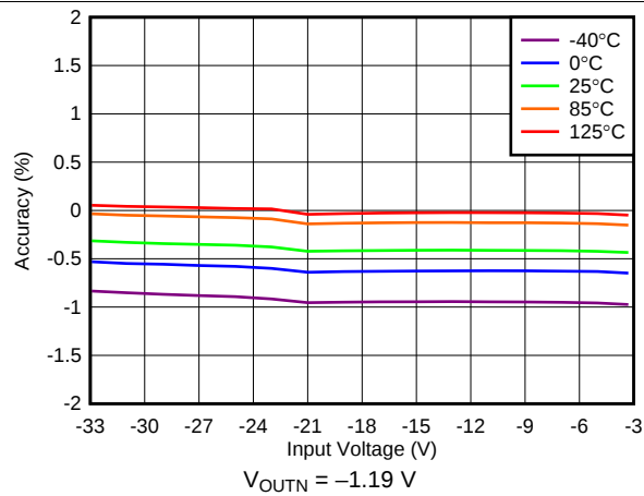
图 34. Negative Line Regulation
