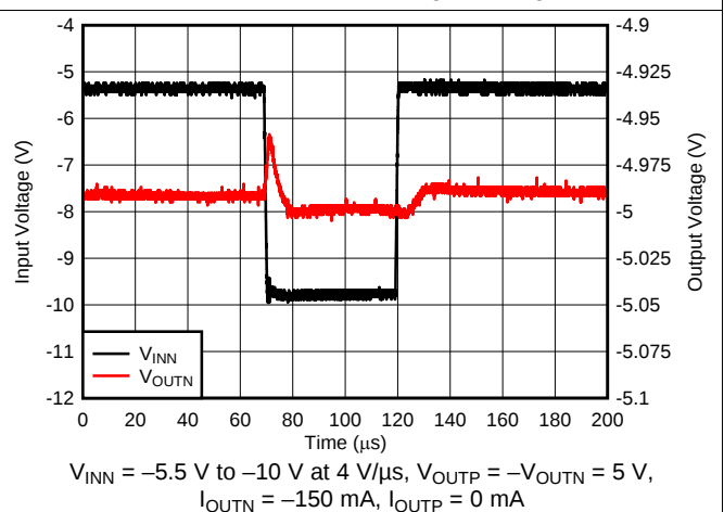
图 29. Line Transient Negative Regulator
