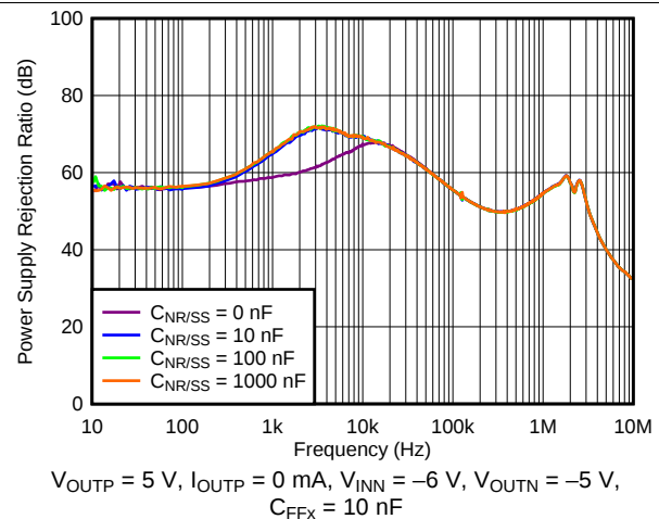
图 11. Negative PSRR vs Frequency and C_{\text{NR/SS}}
