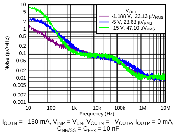
图 15. Negative Spectral Noise Density vs Frequency and V_{\text{OUTN}}
