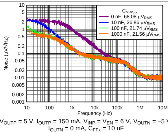
图 16. Positive Spectral Noise Density vs Frequency and C_{\text{NR/SS}}
