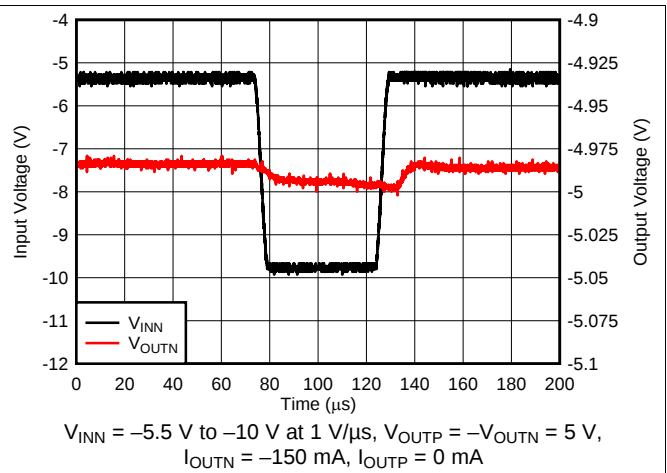
图 27. Line Transient Negative Regulator
