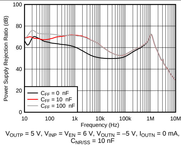
图 8. Positive PSRR vs Frequency and C_{\text{FFP}}
