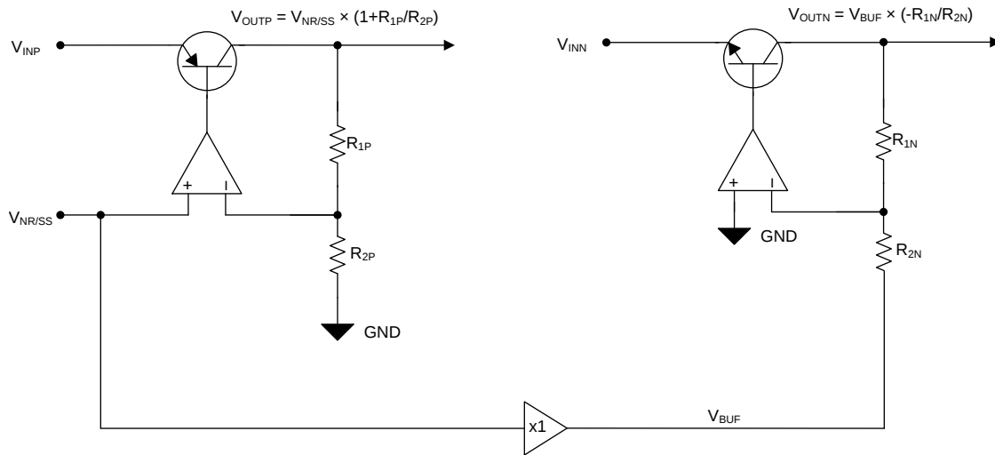
图 63. Simplified Regulation Circuit
