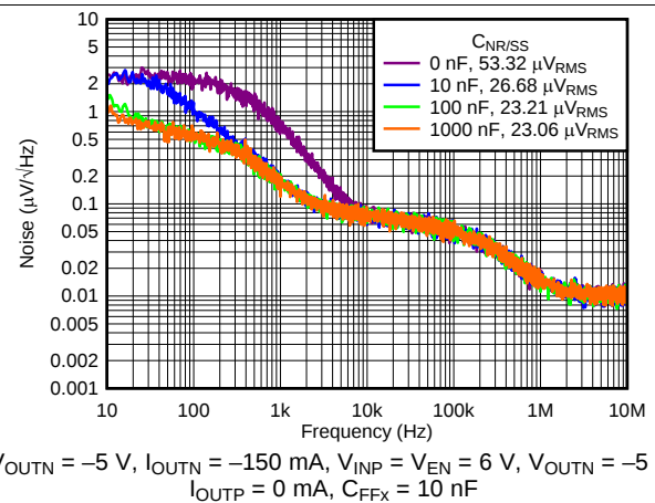
图 17. Negative Spectral Noise Density vs Frequency and C_{\text{NR/SS}}
