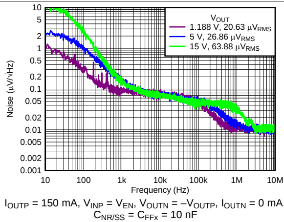
图 14. Positive Spectral Noise Density vs Frequency and V_{\text{OUTP}}
