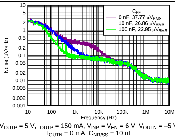
图 18. Positive Spectral Noise Density vs Frequency and C_{\text{FF}}
