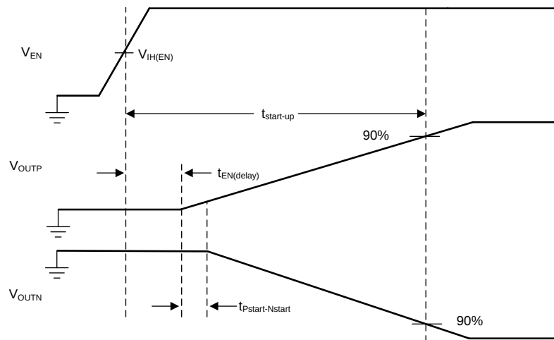
图 1. Start-Up Characteristics
