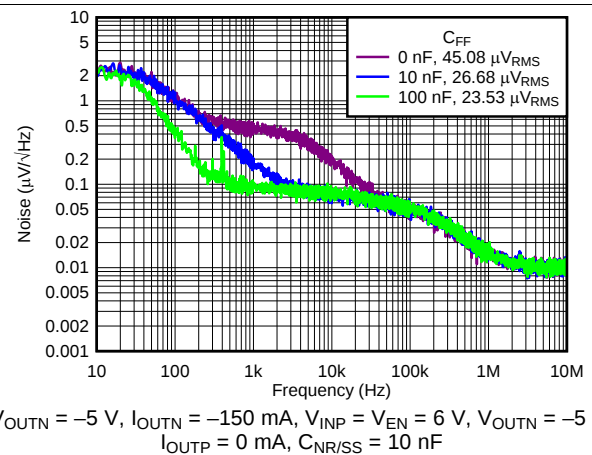
图 19. Negative Spectral Noise Density vs Frequency and C_{\text{FF}}
