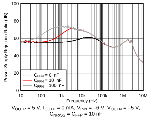
图 9. Negative PSRR vs Frequency and C_{\text{FFN}}
