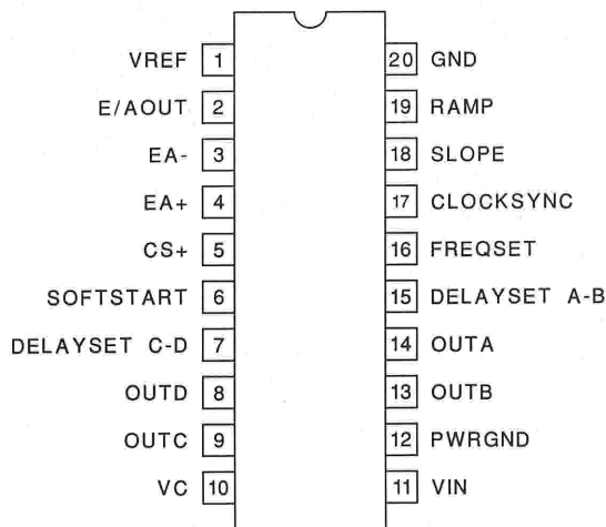
Dip-20 (Top View) J or N Package
