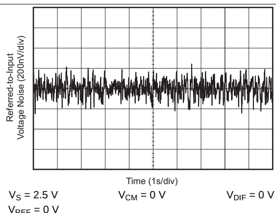
图 16. 0.1-Hz to 10-Hz Voltage Noise (Referred-To-Input)
