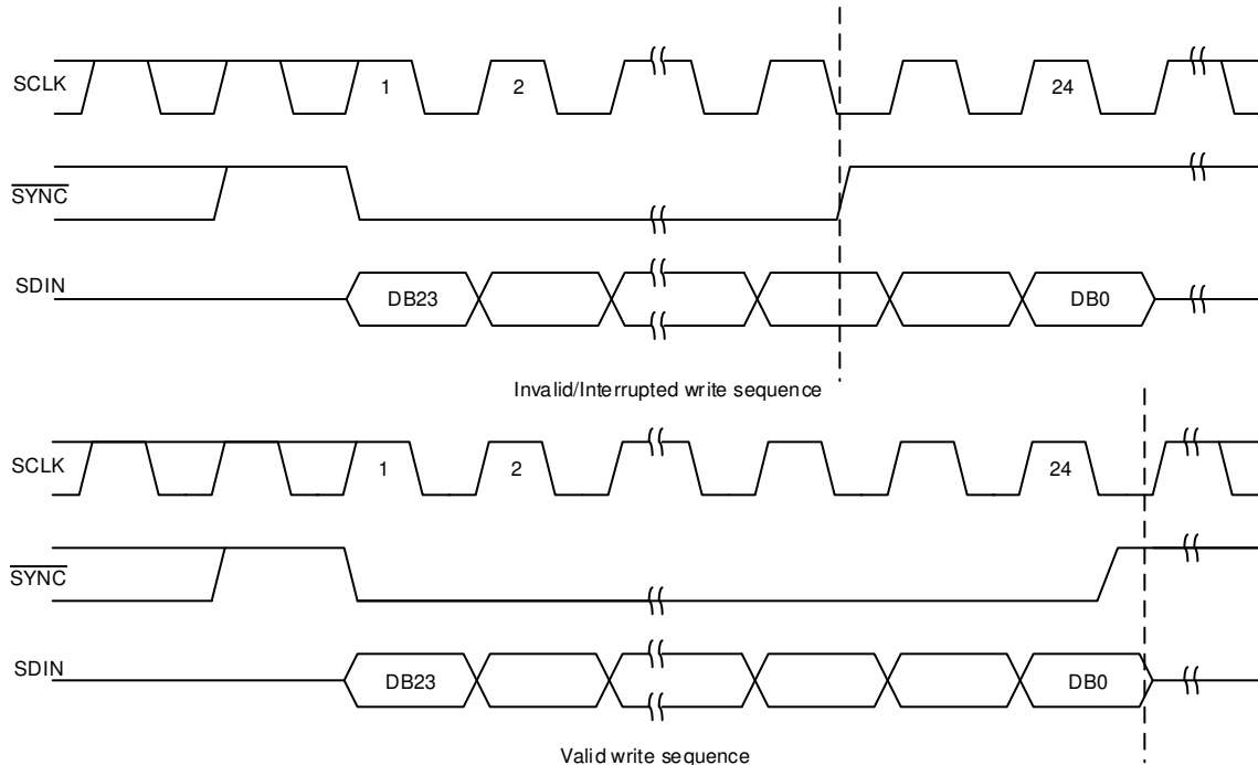
图 58. \overline{\text{SYNC}} Interrupt
