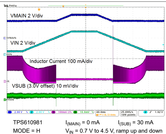
图 9-20. Line Regulation
