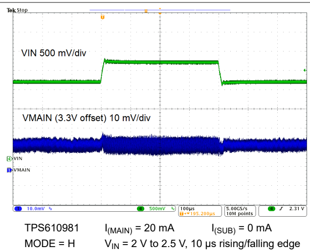
图 9-16. Line Transient Response
