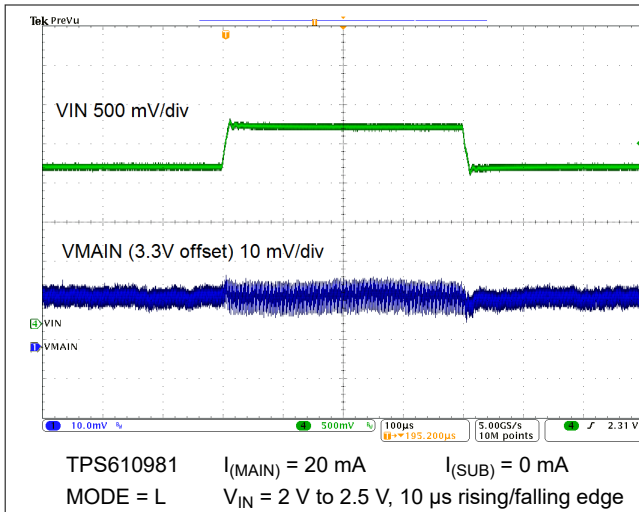
图 9-15. Line Transient Response
