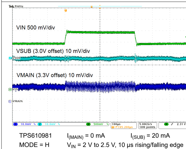
图 9-17. Line Transient Response
