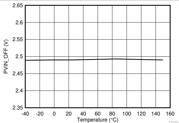
图 6-14. Turnoff Voltage vs Junction Temperature
