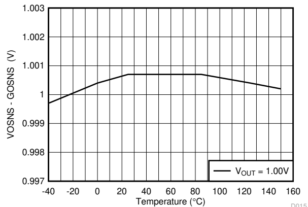
图 6-8. Output Voltage vs Junction Temperature
