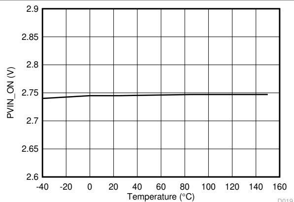
图 6-13. Turnon Voltage vs Junction Temperature
