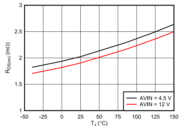
图 6-6. Low-Side MOSFET On-Resistance ( R_{DS(on)} ) vs Junction Temperature
