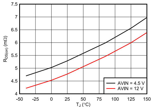
图 6-7. High-Side MOSFET On-Resistance ( R_{DS(on)} ) vs Junction Temperature
