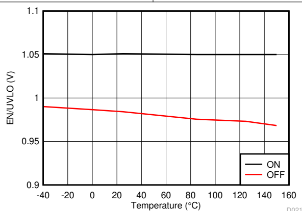
图 6-15. EN/UVLO Thresholds vs Junction Temperature
