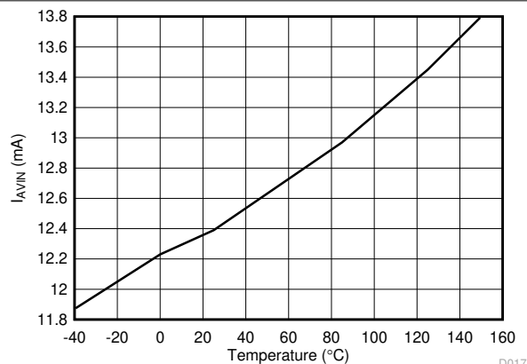
图 6-10. Non-Switching Input Current ( I_{AVIN} ) vs Junction Temperature
