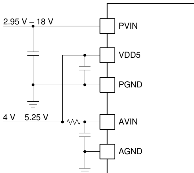
图 7-3. TPS546A24A Separate PVIN and AVIN connections with VDD5
