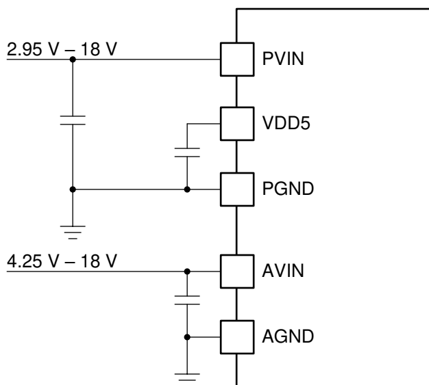
图 7-2. TPS546A24A Separate PVIN and AVIN connections
