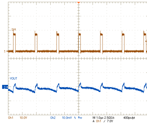
图 8-8. V_{OUT} Steady-State Ripple
