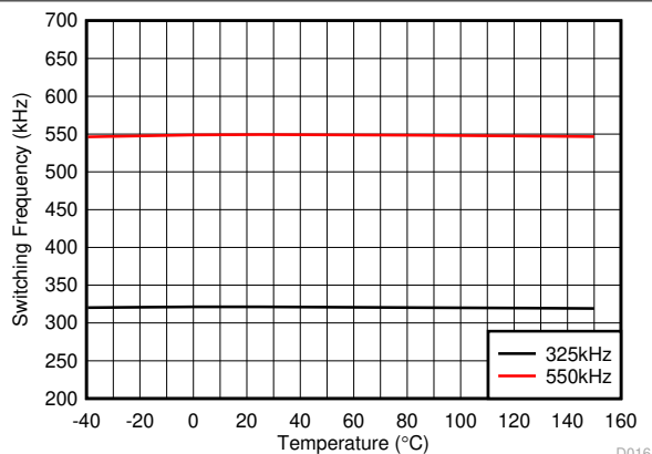
图 6-9. Switching Frequency vs Junction Temperature
