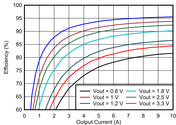
图 6-5. TPS546A24A Efficiency vs Output Current
