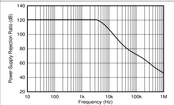
图 6-12. Power-Supply Rejection Ratio vs Frequency
