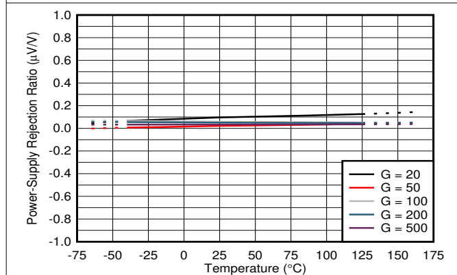
图 6-11. Power-Supply Rejection Ratio vs Temperature
