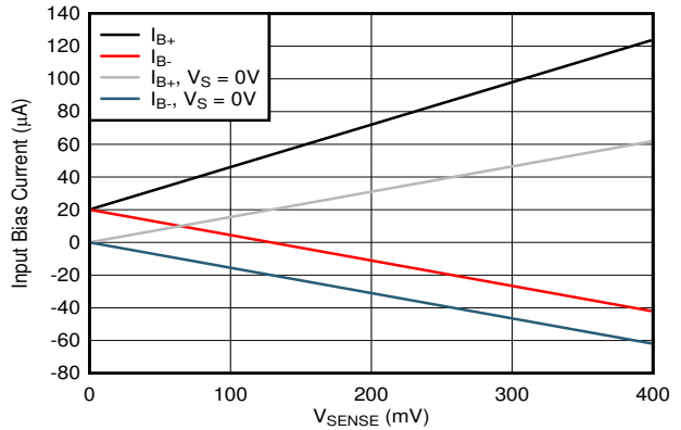
图 6-16. INA293x2Q, INA293x3Q Input Bias Current vs V_{\text{SENSE}}
