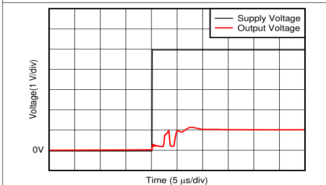
图 6-33. Start-Up Response
