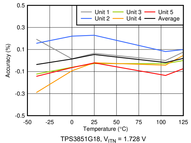
图 6-6. V_{ITN} + V_{HYS} Accuracy vs Temperature TPS3851G18, V_{ITN} = 1.728\text{ V}
