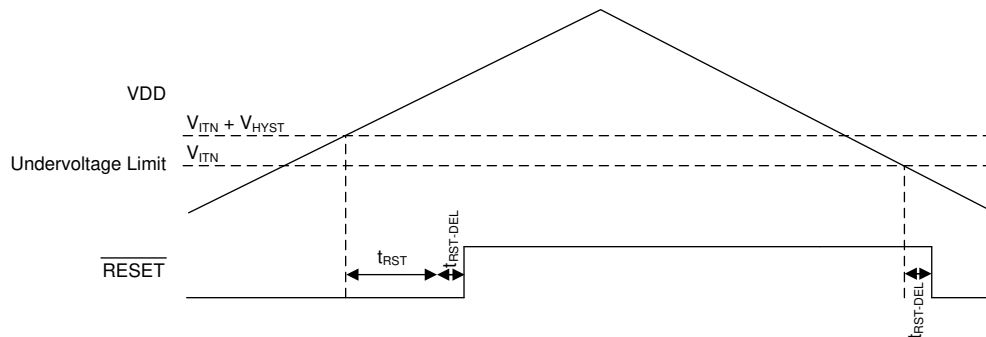
图 7-1. Undervoltage Detection
