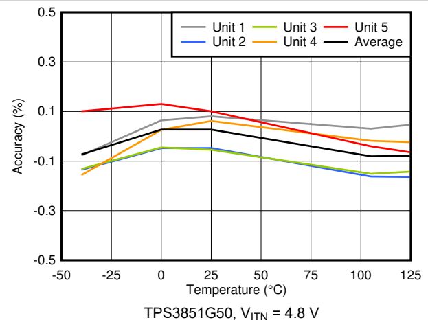
图 6-8. V_{ITN} + V_{HYS} Accuracy vs Temperature TPS3851G50, V_{ITN} = 4.8\text{ V}
