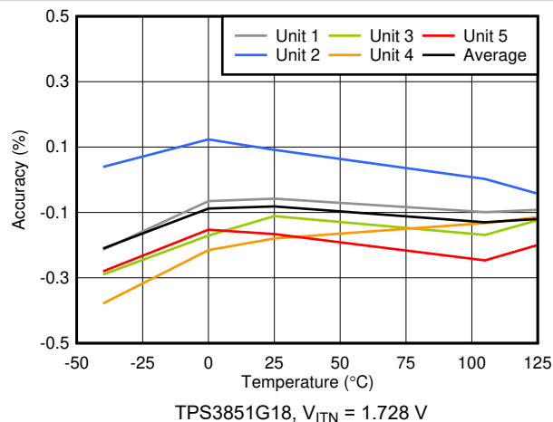
图 6-7. V_{ITN} Accuracy vs Temperature TPS3851G18, V_{ITN} = 1.728\text{ V}
