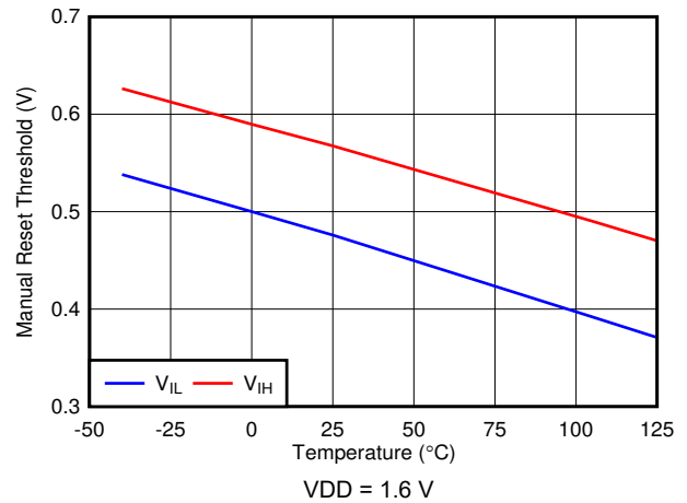
图 6-4. \overline{MR} Threshold vs Temperature V_{DD} = 1.6\text{ V}
