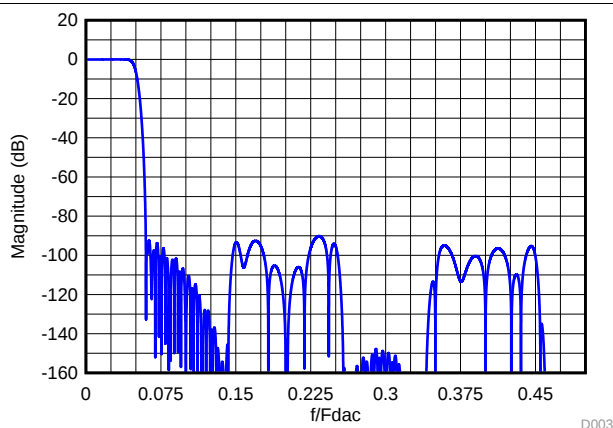
Figure 44. Composite Magnitude Response for 10x Interpolation
