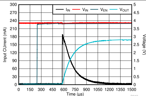
图 6-82. Start-Up
