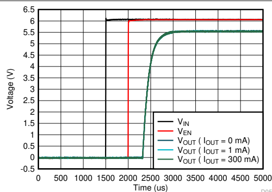
图 6-80. Start-Up
