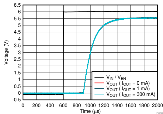
图 6-80. Start-Up
