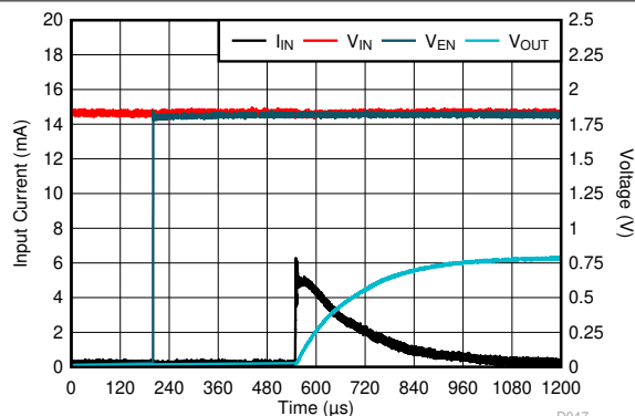
图 6-81. Start-Up
