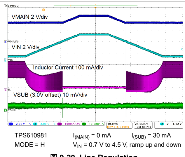
图 9-20. Line Regulation
