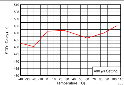
图 7-12. Short Circuit Discharge 1 Delay Time vs. Temperature
