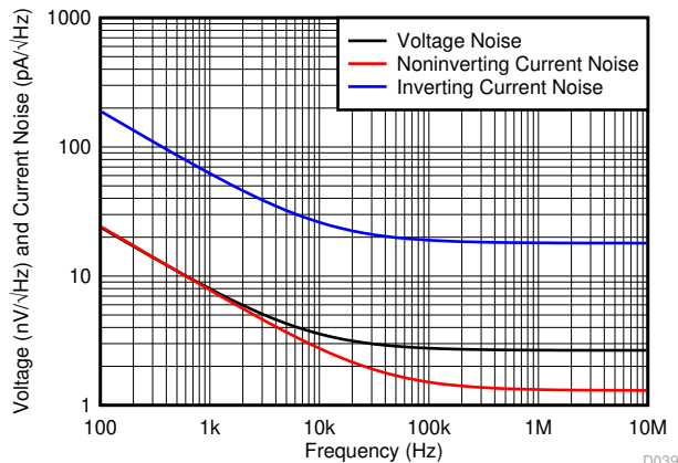
图 6-39. Input-Referred Spot Noise vs Frequency
