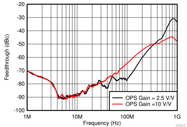
图 8-13. Forward Feedthrough With OPS Enabled, External Path Selected
