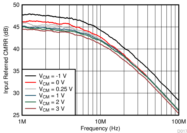
图 6-17. Common-Mode Rejection Ratio vs Input Common-Mode Voltage
