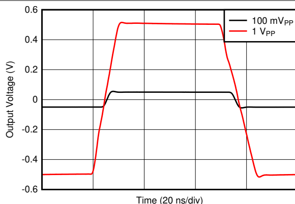
图 6-50. Step Response
