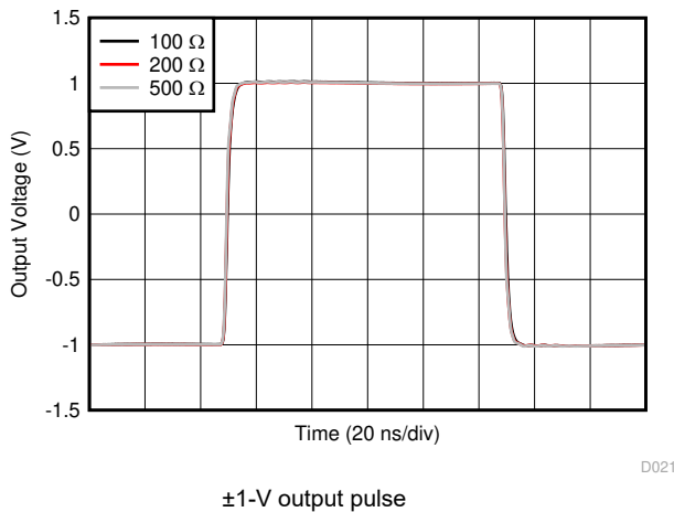
图 6-21. Large-Signal Step Response vs Load Resistance
