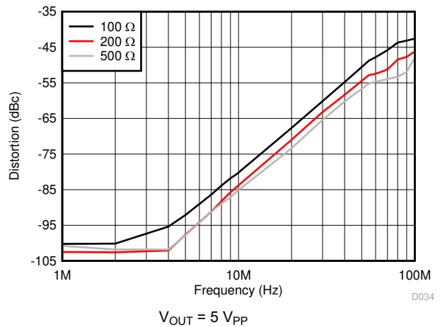
图 6-34. HD3 vs Load Resistance
