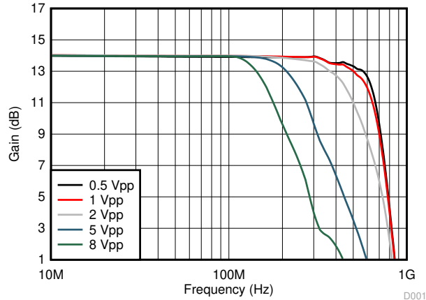
图 6-1. Frequency Response vs Output Voltage
