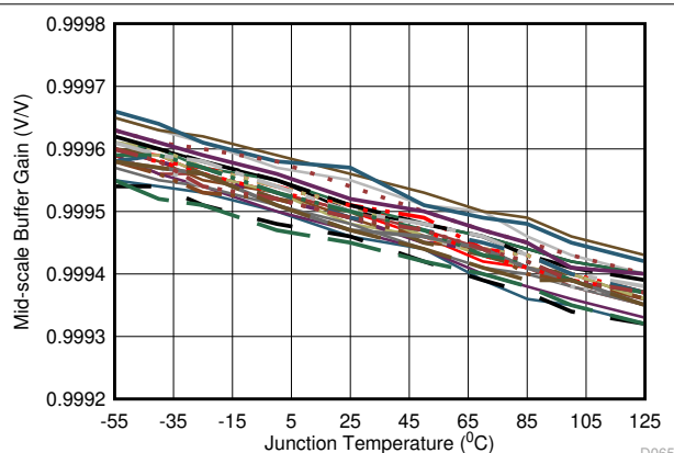
图 6-63. OPS Gain Over Temperature
