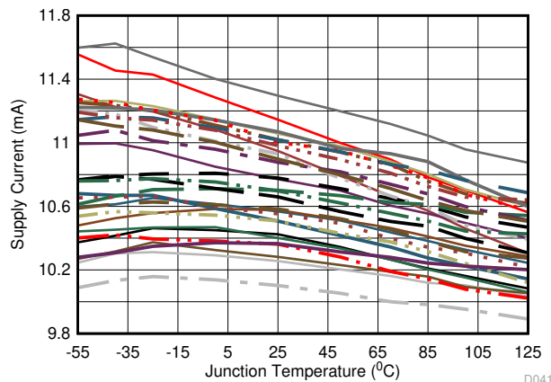
图 6-41. Quiescent Supply Current vs Temperature
