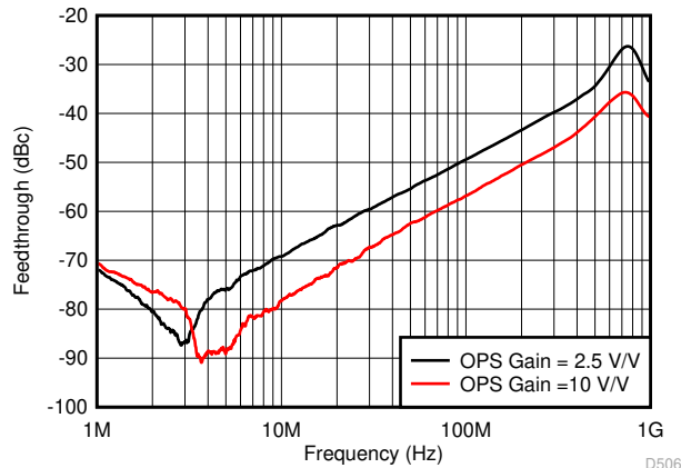
图 8-12. Forward Feedthrough With OPS Enabled, Internal Path Selected
