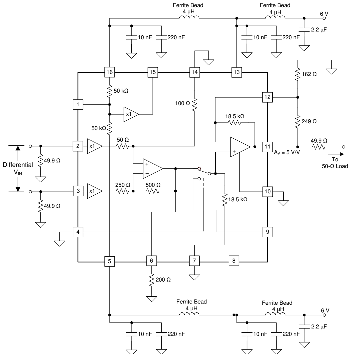
图 10-1. Recommended Power-Supply Configuration
