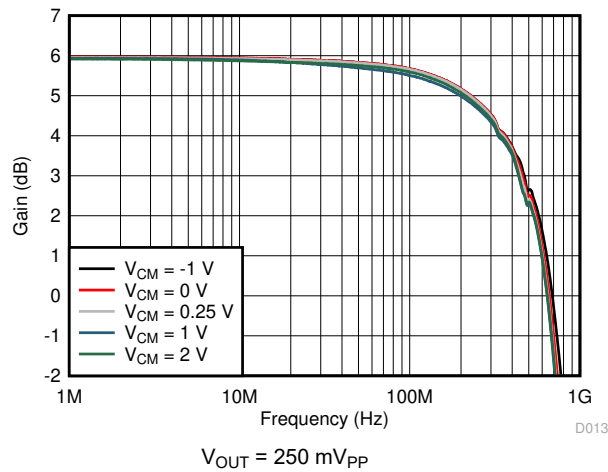
图 6-13. Frequency Response vs Input Common-Mode Voltage
