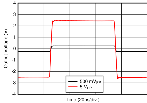
图 6-2. Small- and Large-Signal Step Response
