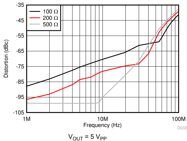
图 6-33. HD2 vs Load Resistance
