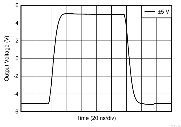
图 9-8. Pulse Response of the System With the Interstage Bessel Filter
