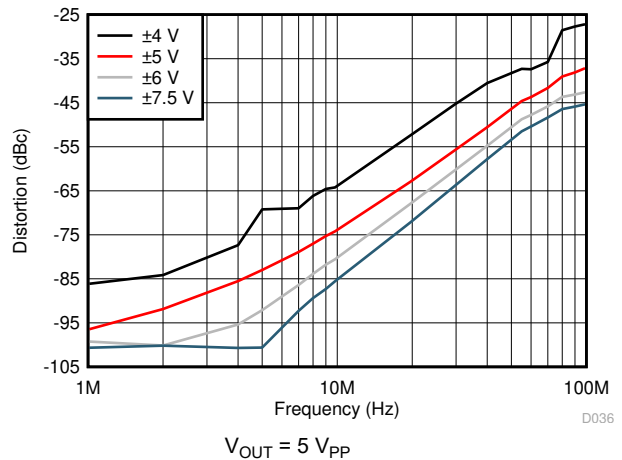
图 6-36. HD3 vs Supply Voltage
