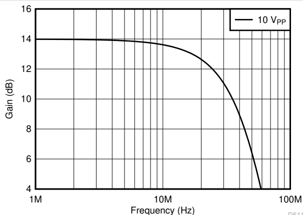
图 9-7. Frequency Response of the System With the Interstage Bessel Filter
