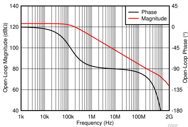
图 8-7. Simulated OPS Z OL Gain Magnitude and Phase
