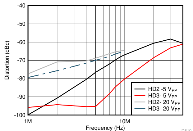
图 9-5. Harmonic Distortion Performance of the 5 V PP and 20 V PP Channels
