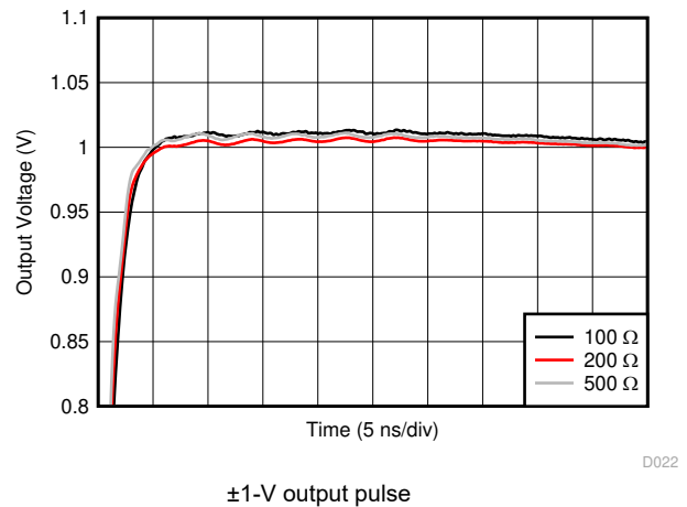
图 6-22. Large-Signal Pulse Settling Response vs Load Resistance
