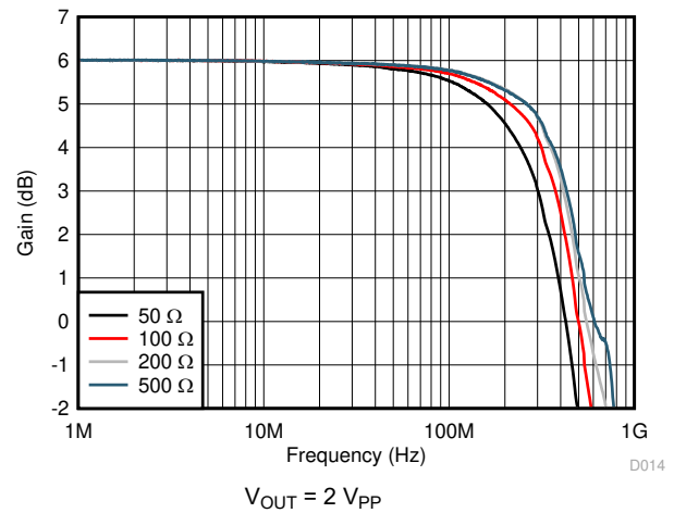
图 6-14. Frequency Response vs Load Resistance
