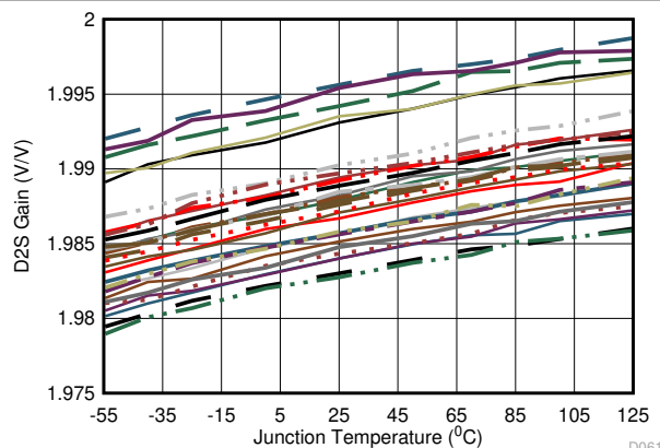
图 6-61. D2S Gain Over Temperature
