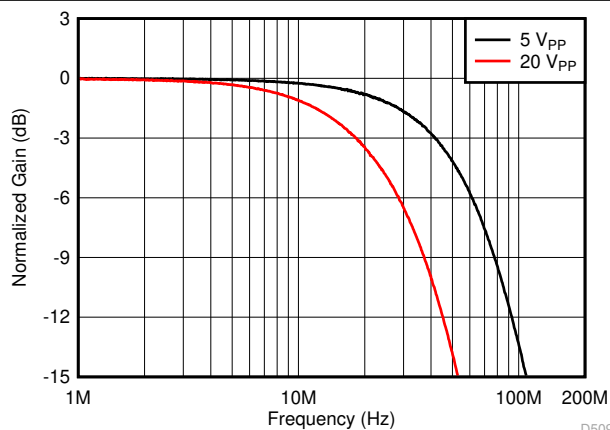
图 9-4. Frequency Response of the 5 V PP and 20 V PP Channels
