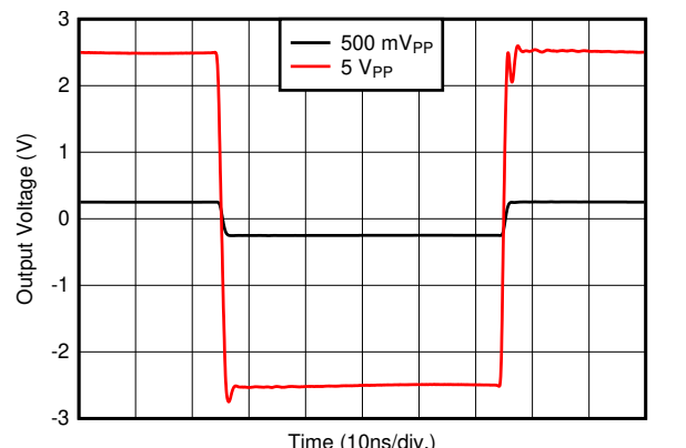
图 6-28. Inverting Response vs Output Voltage
