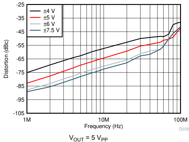
图 6-35. HD2 vs Supply Voltage
