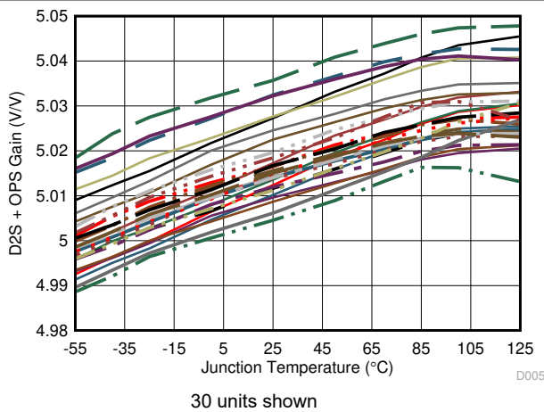
图 6-5. Gain vs Temperature
