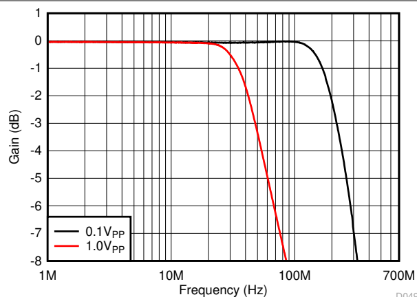
图 6-49. Frequency Response vs Output Voltage
