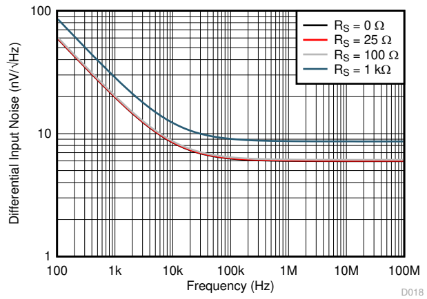
图 6-18. Differential Input Noise vs Source Impedance
