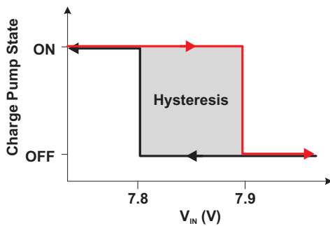
Figure 19. Charge Pump Operation at Light Loads
