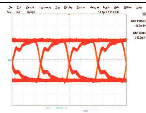
Figure 27. Typical Eye Pattern SN65LVDS180: Tx + Rx
