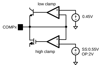
Figure 23. Error Flag Operation
