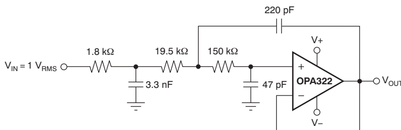
Figure 38. OPA322 Configured as a Three-Pole, 20-kHz, Sallen-Key Filter
