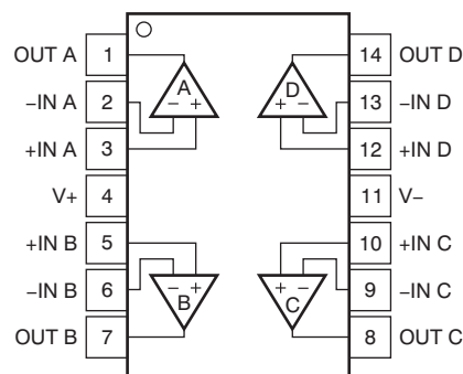
PW PACKAGE TSSOP-14 (TOP VIEW)
