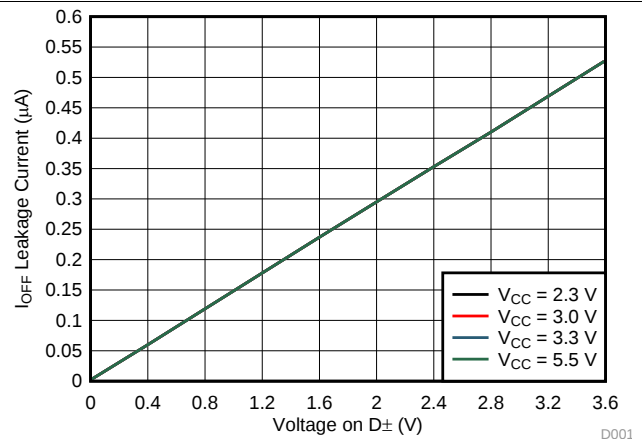
图 2. I_{OFF} Leakage Current vs Voltage on D^\pm
