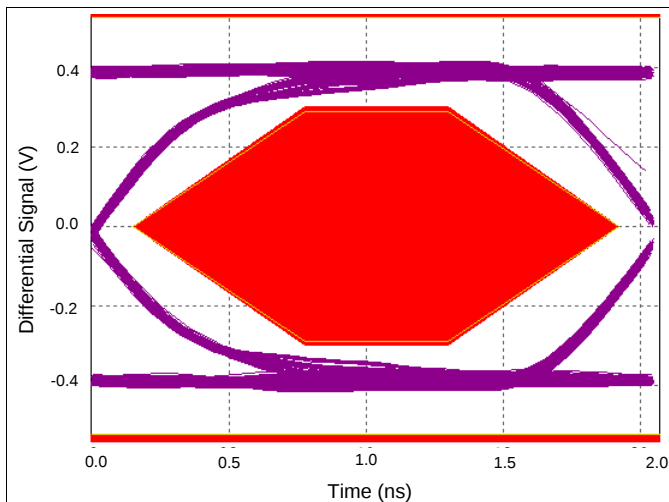
图 21. High Speed Eye Diagram With TS5USBC41
