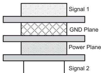
图 23. Four-Layer Board Stack-Up
