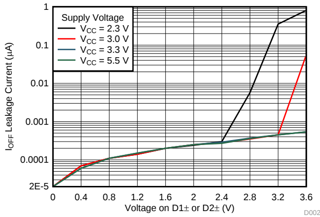
图 3. I_{OFF} Leakage Current vs Voltage on D1^\pm or D2^\pm
