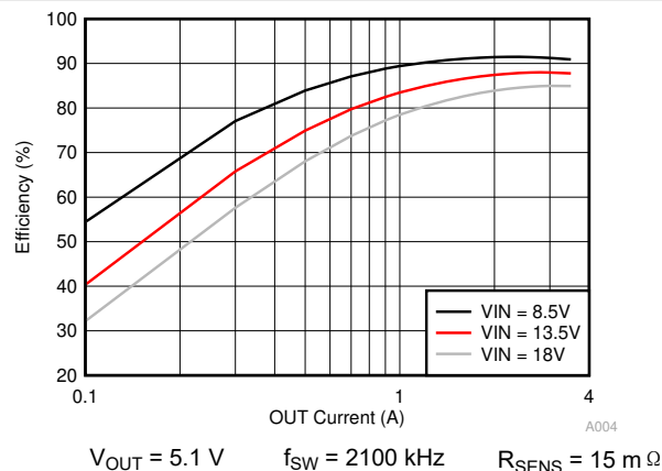
图 11-5. Efficiency with Sense Resistor
