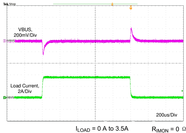
图 11-8. Load Transient Without Cable Compensation
