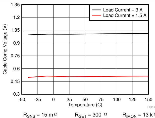
图 8-17. Cable Compensation Voltage vs Junction Temperature
