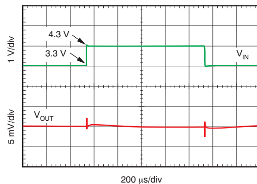
Figure 29. Line Transient Response V_{OUT} = 1.8 \text{ V} , I_{OUT} = 500 \text{ mA}
