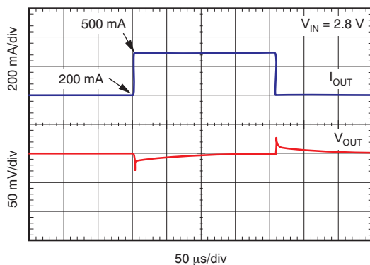
Figure 28. Load Transient Response 200 mA to 500 mA, C_{OUT} = 1 \mu\text{F}
