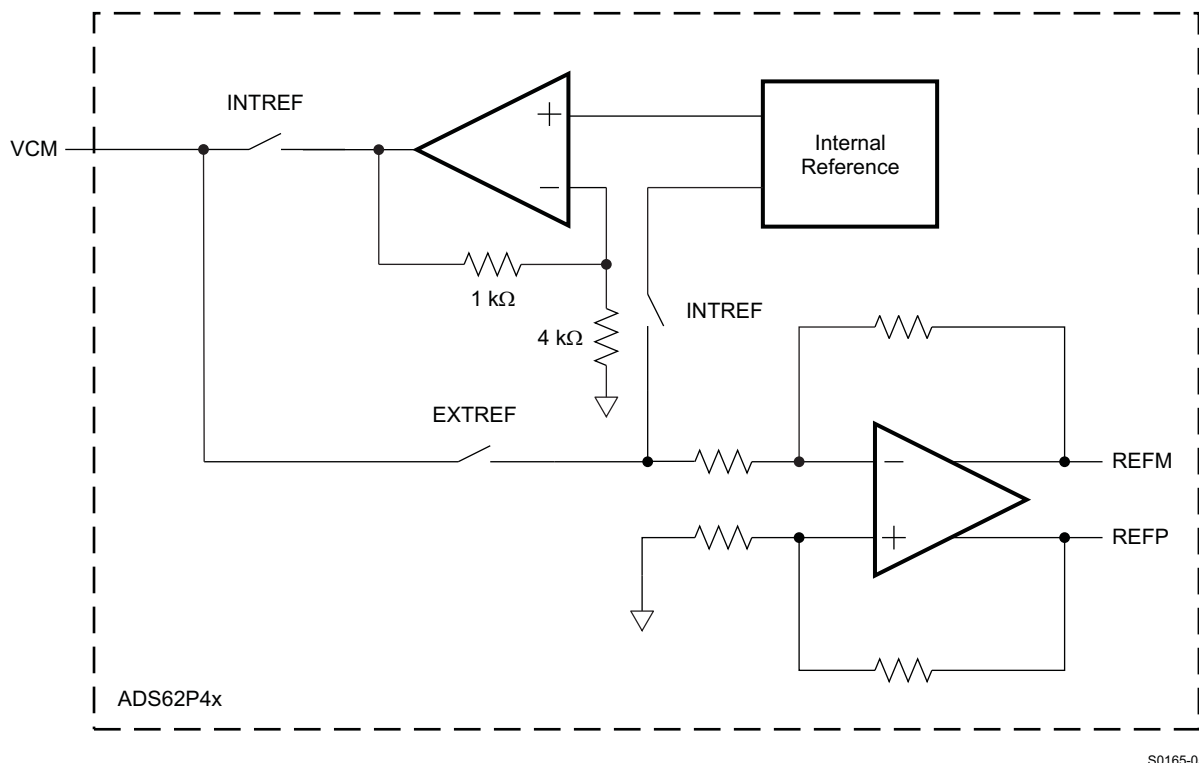
Figure 89. Reference Section
