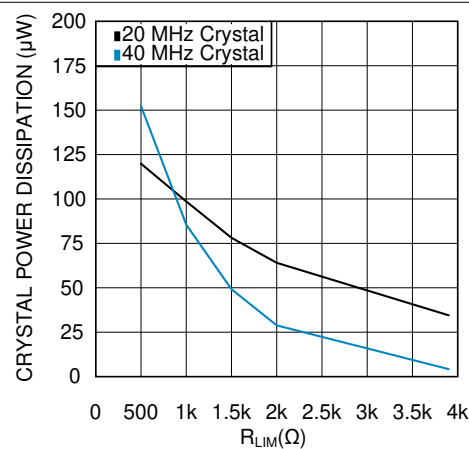
图 6-10. Crystal Power Dissipation vs. R_{LIM}
