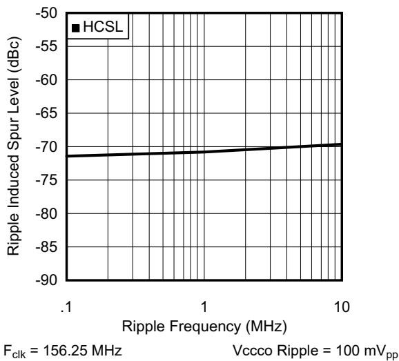
图 6-7. PSRR vs. Ripple Frequency at 156.25 MHz
