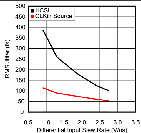
图 6-6. RMS Jitter vs. CLKin Slew Rate at 156.25 MHz
