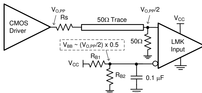
图 9-3. Single-Ended LVCMOS Input, DC Coupling With Common-Mode Biasing
