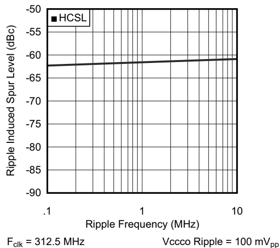
图 6-8. PSRR vs. Ripple Frequency at 312.5 MHz
