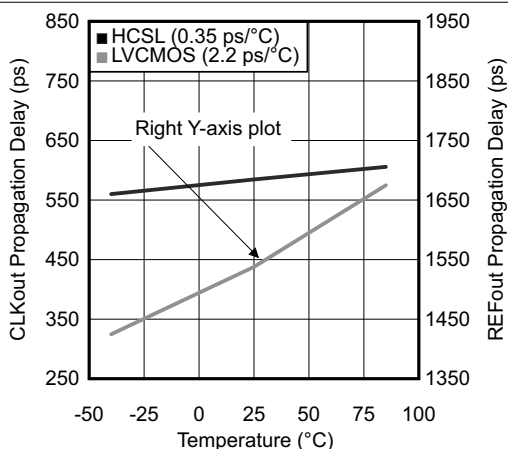
图 6-9. Propagation Delay vs. Temperature
