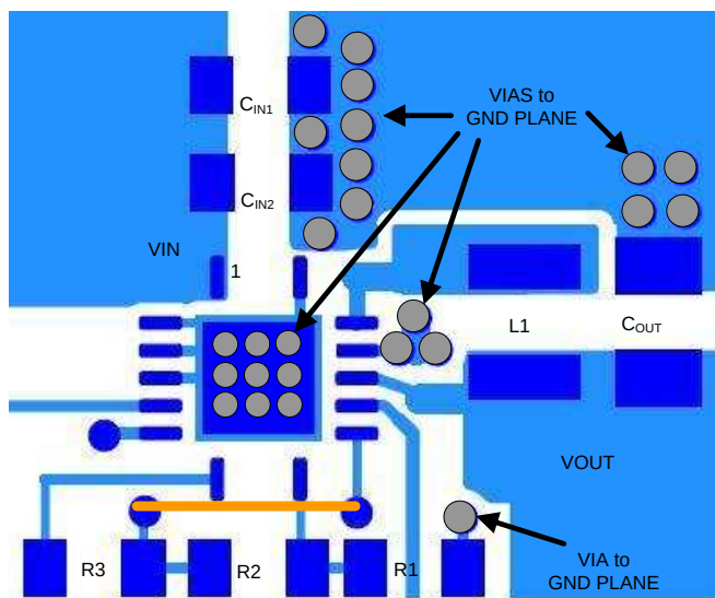
Figure 74. Recommended Layout, TPS62736
