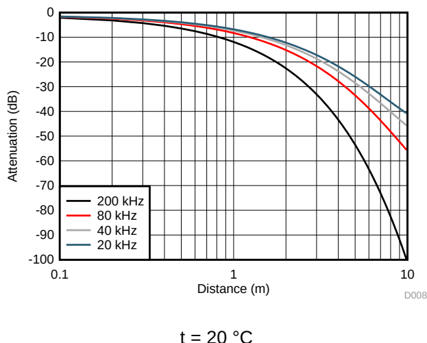
图 137. Attenuation Characteristics of Sound Pressure by Distance
