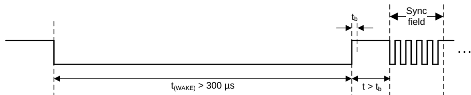
图 38. USART Wake-Up Pulse
