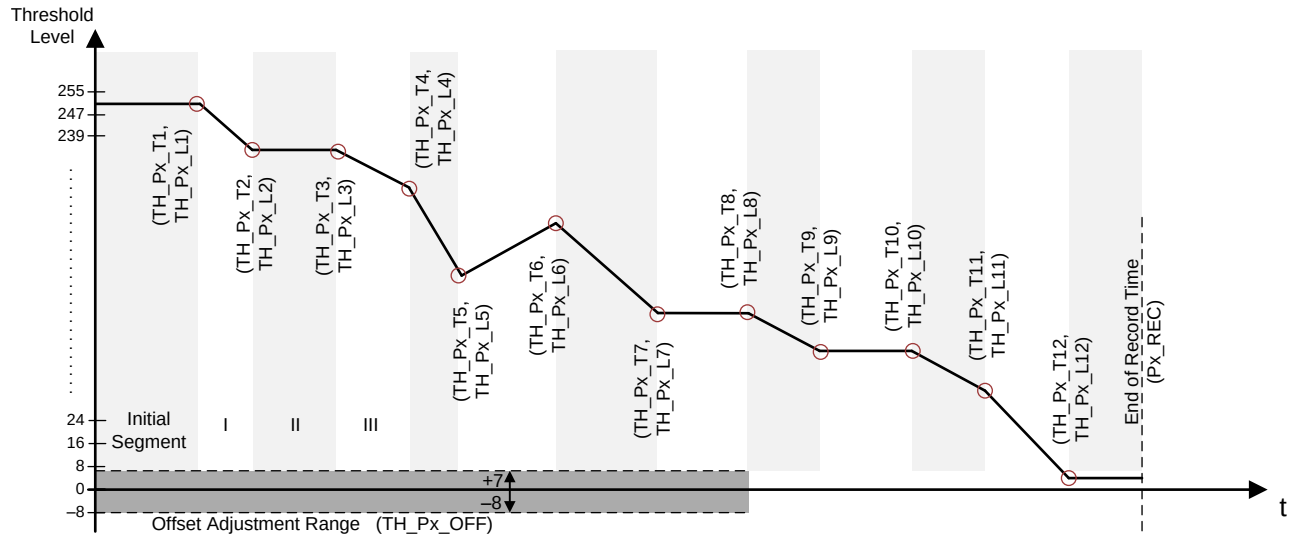
图 8. Threshold Assignment Example
