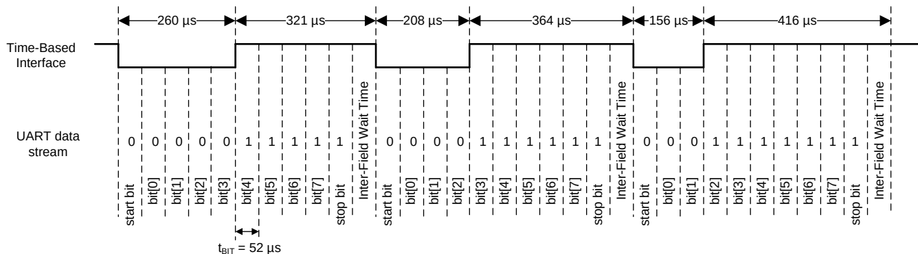
图 34. IO-Pin Interface Toggle Pattern
