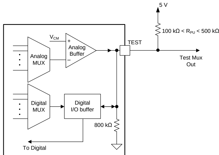
图 42. Test Pin Test Mux Output Application
