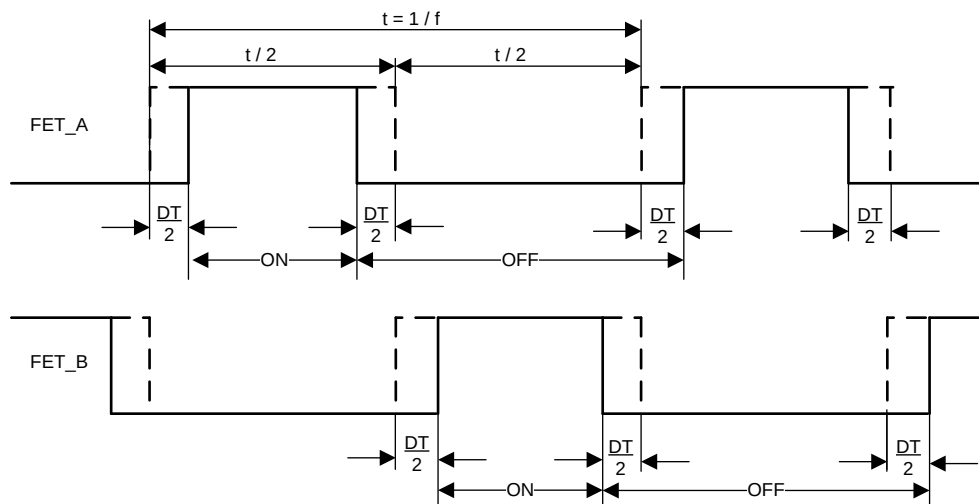
图 4. Echo Generation Dead-Time Adjustment
