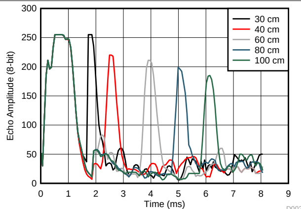
图 140. Short Range ISO-Pole Measurements Using Transformer Drive
