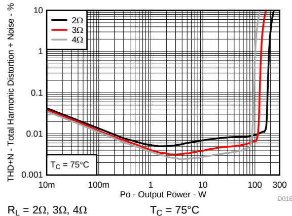
图 16. Total Harmonic Distortion+Noise vs Output Power
