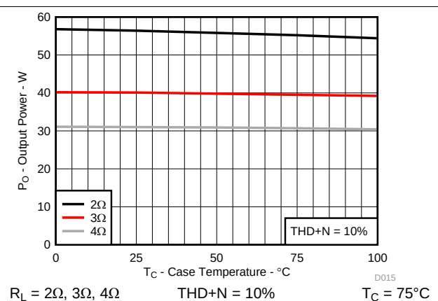
图 15. Output Power vs Case Temperature
