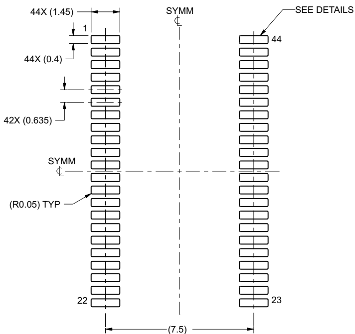
LAND PATTERN EXAMPLE SCALE:6X
