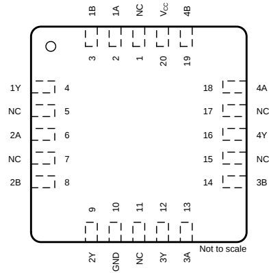
SN54LVC32A FK Package 20-Pin LCCC Top View
