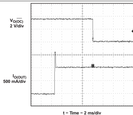
Figure 55. 3-Ω Load Connected to Enabled Device
