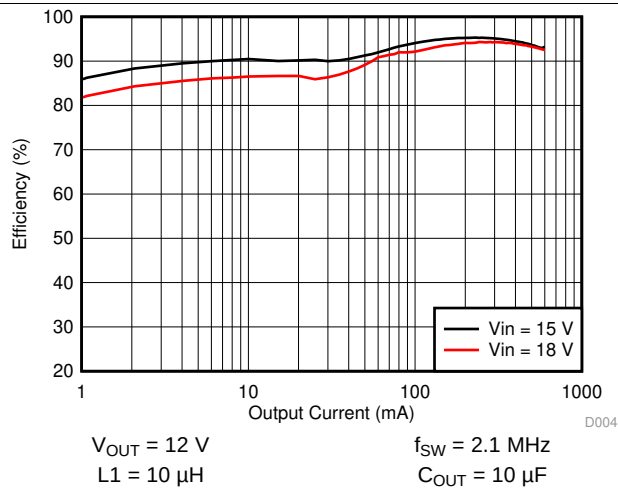
Figure 3. Efficiency versus Load Current
