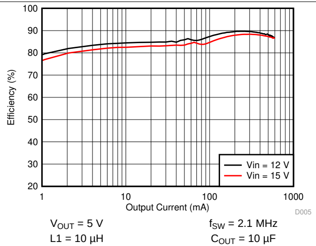
Figure 4. Efficiency versus Load Current
