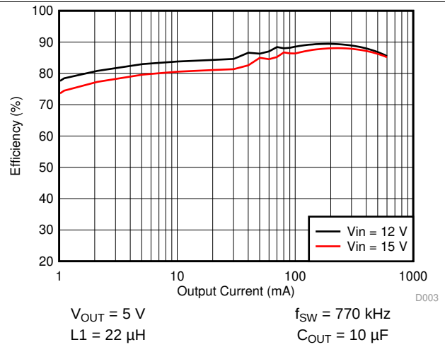
Figure 2. Efficiency versus Load Current
