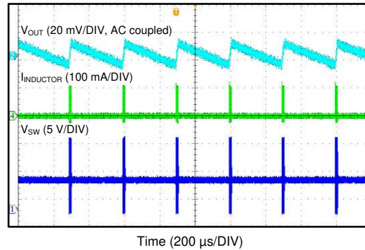
Figure 14. ECO Mode Operation
