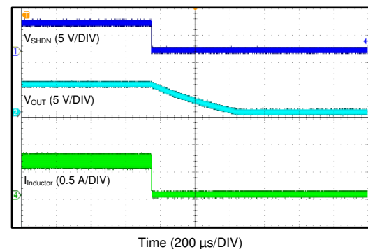
Figure 11. Shutdown Waveform
