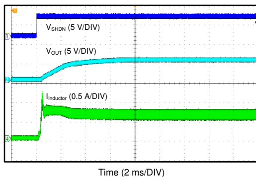
Figure 10. Start-up Waveform
