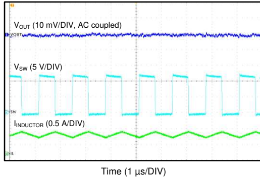
Figure 8. Switching Node and Output Voltage Waveform
