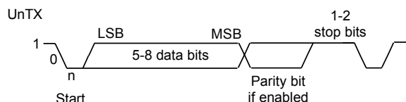
Figure 16-2. UART Character Frame
