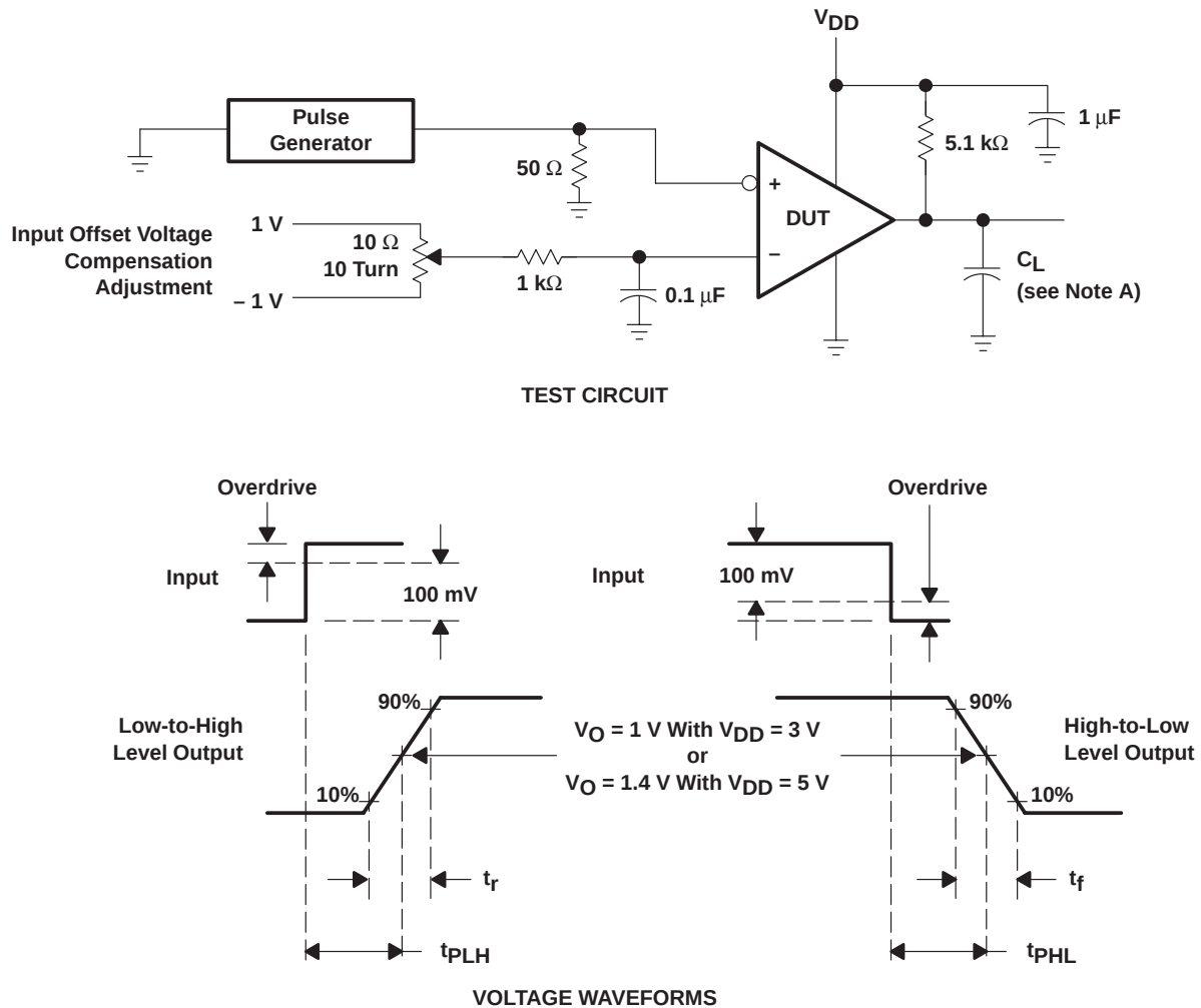
Figure 11. Propagation Delay, Rise, and Fall Times Test Circuit and Voltage Waveforms
