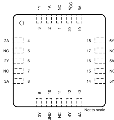
LCCC Package 20-Pin FK Top View
