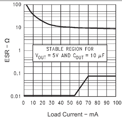
Figure 6. 5-V/10- \mu\text{F} ESR Curves
