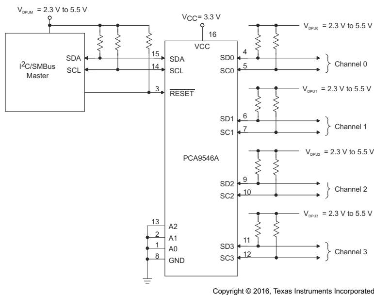
图 9-1. PCA9546A Typical Application Schematic
