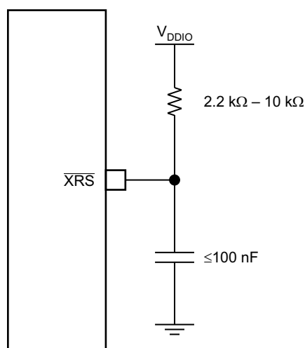
Figure 5-4. Reset Circuit
