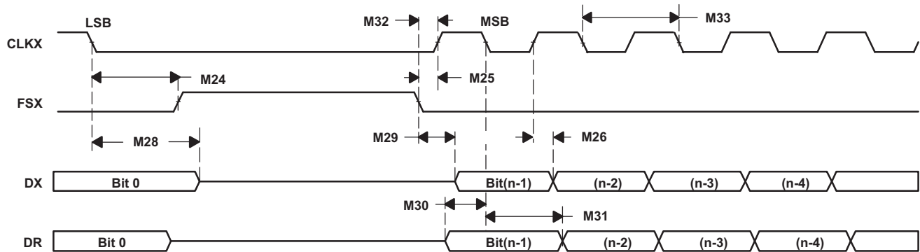
图 5-61. McBSP Timing as SPI Master or Slave: CLKSTP = 10b, CLKXP = 0
