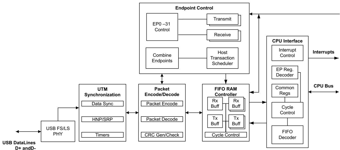
图 5-71. USB Block Diagram
