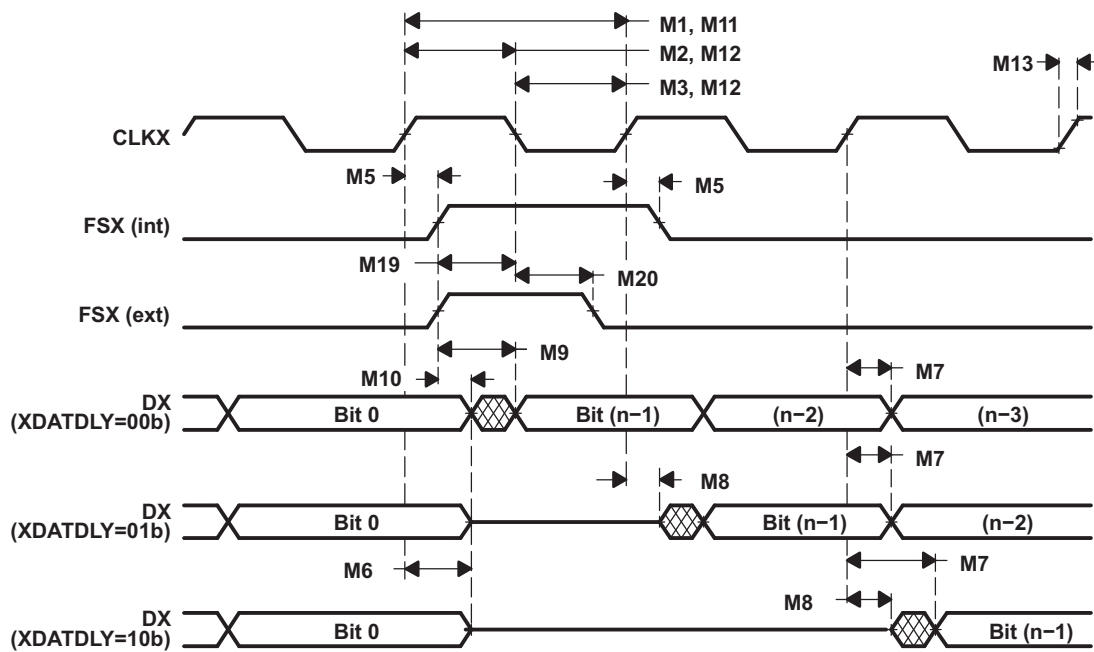
图 5-60. McBSP Transmit Timing
