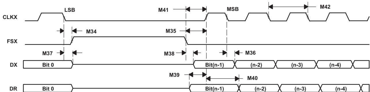
图 5-62. McBSP Timing as SPI Master or Slave: CLKSTP = 11b, CLKXP = 0
