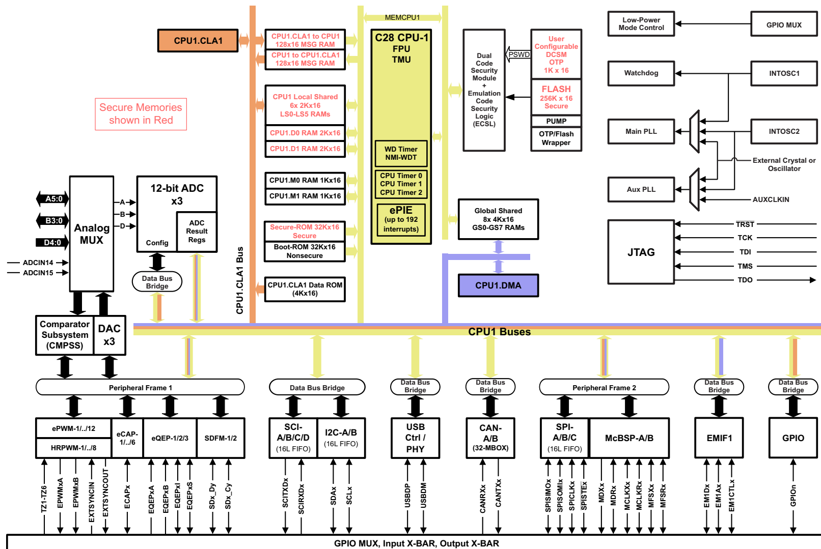
图 6-1. Functional Block Diagram
