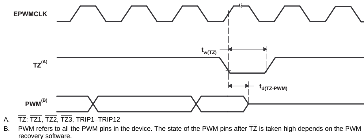
Figure 5-48. PWM Hi-Z Characteristics
