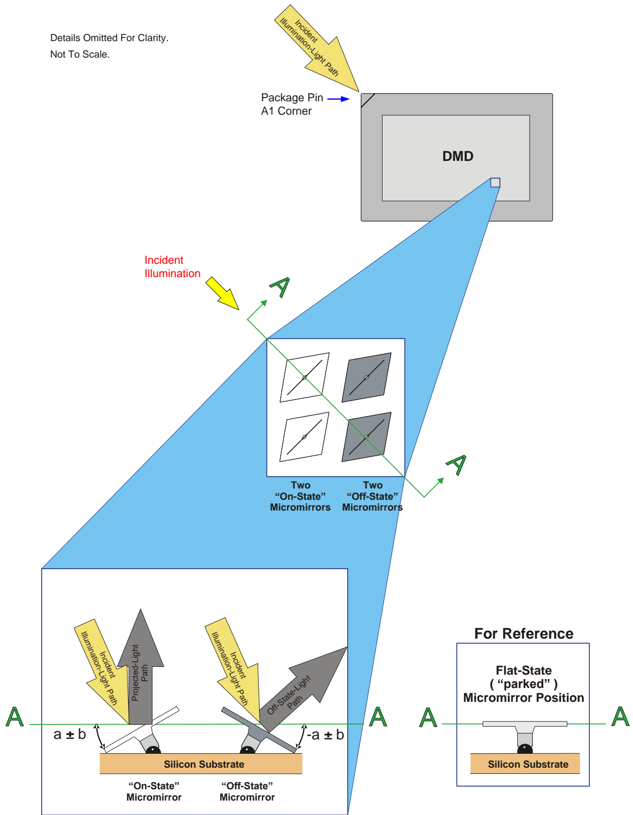
Micromirror States: On, Off, Flat
