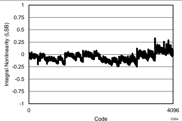
Figure 73. Typical INL
