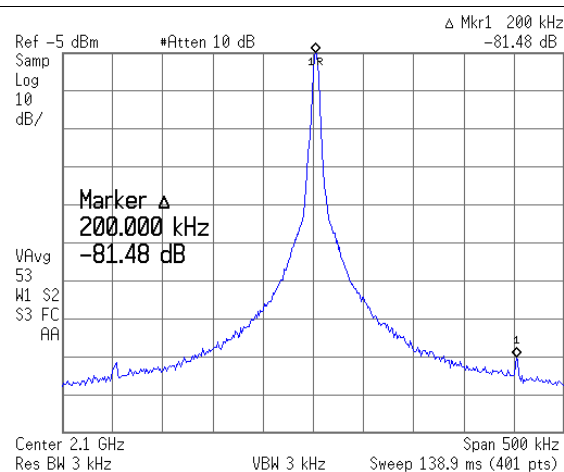
Figure 71. Direct Output: PFD Frequency Spurs
