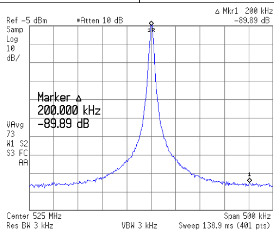
Figure 73. Divide-By-4 Output: PFD Frequency Spurs
